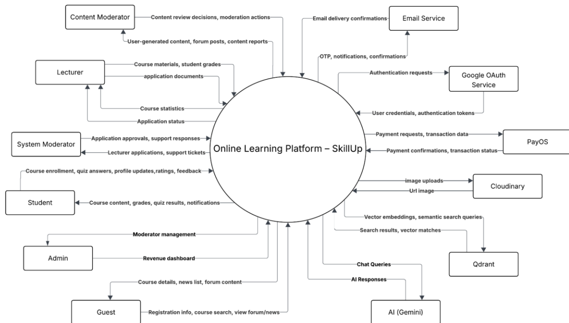
Figure 1.1 - Context diagram of OLP-SkillUp
