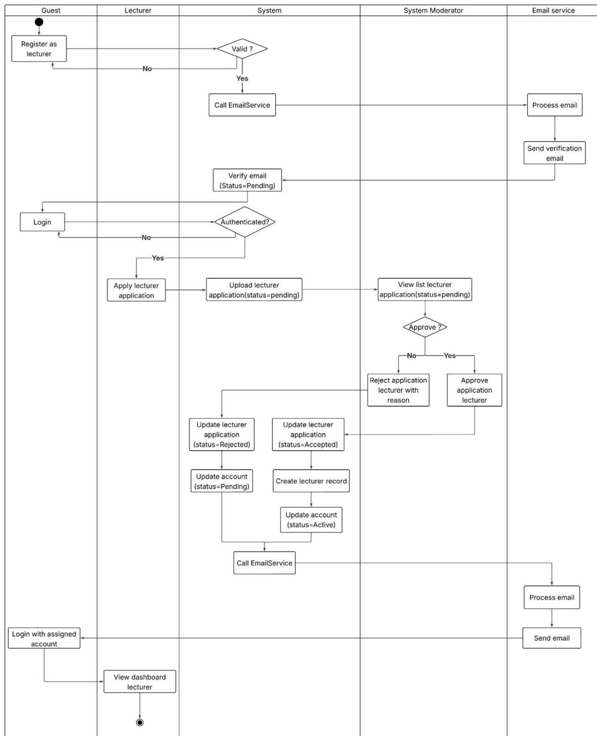
Figure 1.2.1 - Main workflow register to become a lecturer
