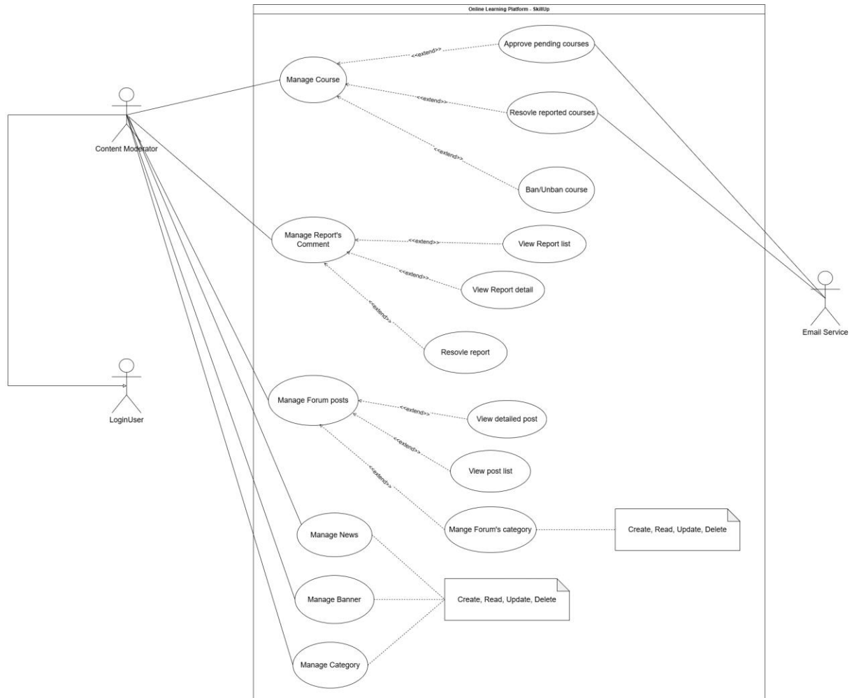
Figure 1.3.3.5 - use case content moderator diagram
