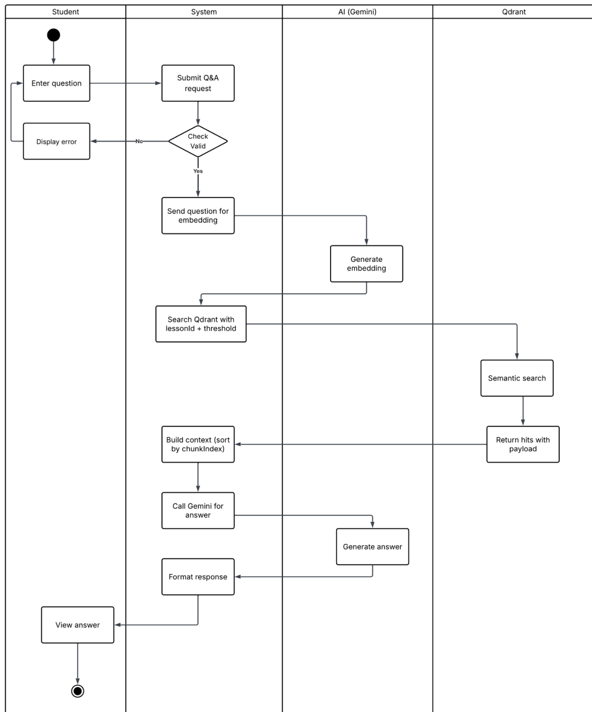
Figure 1.2.5 - Main workflow AI lesson Q&A
