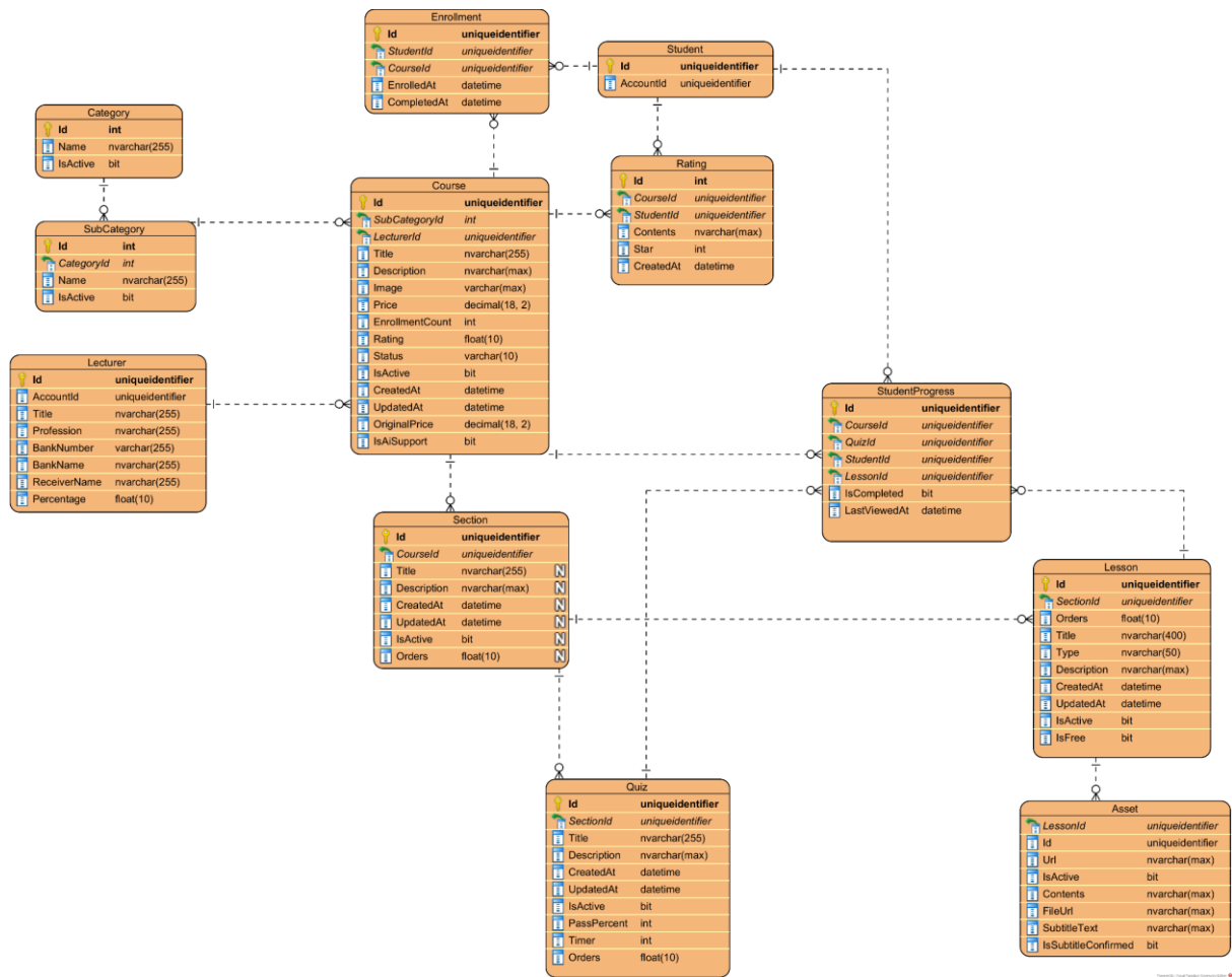
Figure 1.5.3 - Course relationship diagram
