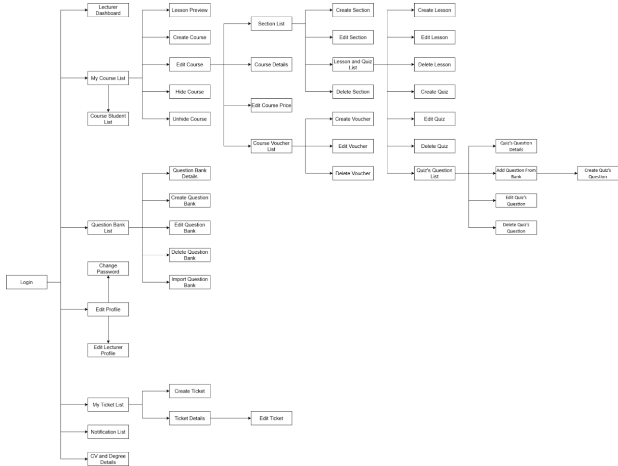
Figure 1.4.1.3 - Lecturer Screens Flow
