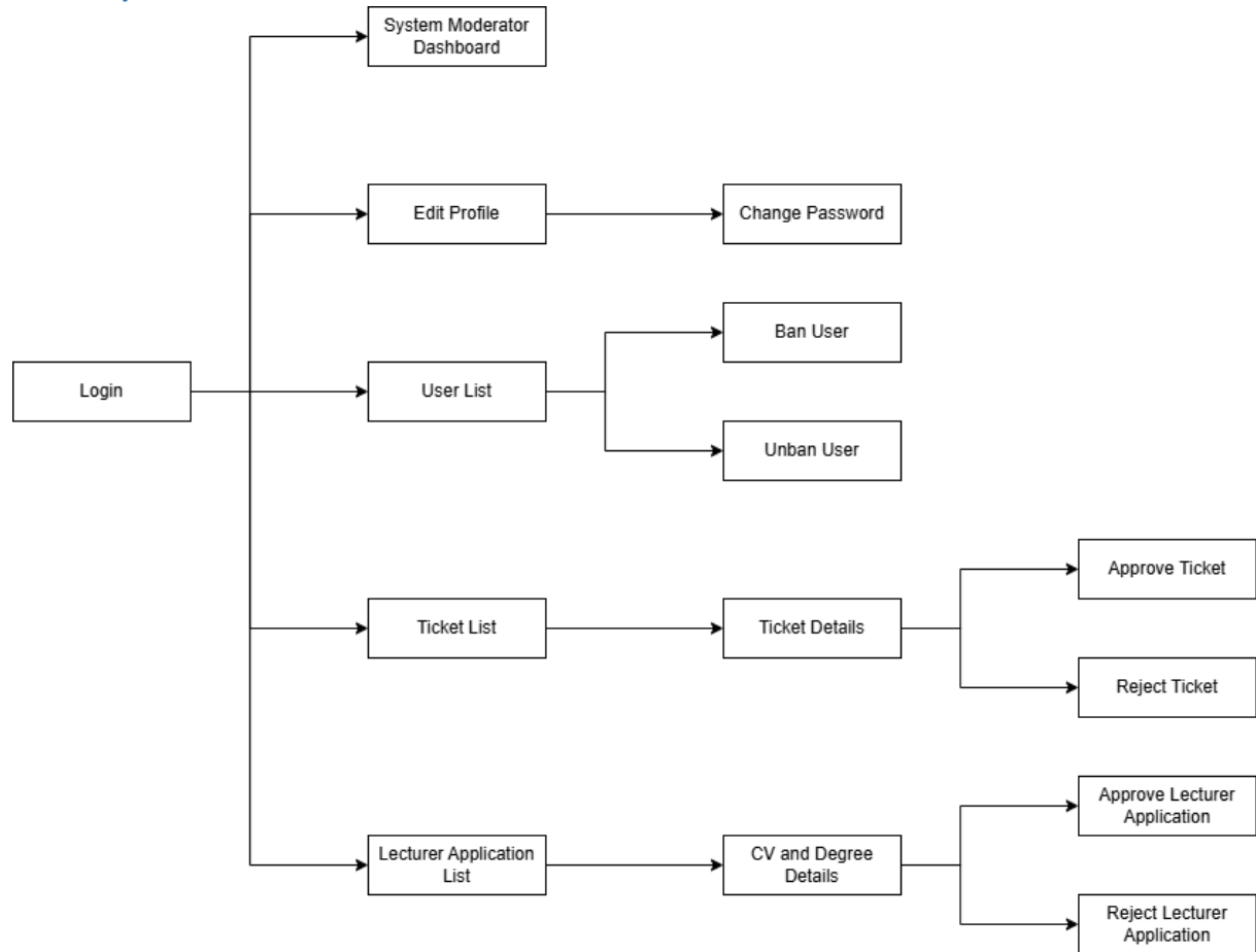
Figure 1.4.1.5 - System moderator Screens Flow
