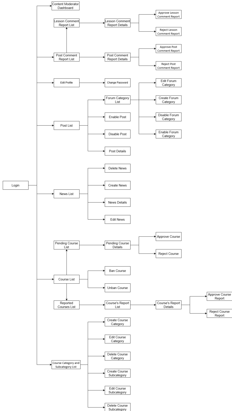
Figure 1.4.1.2 - Content moderator Screens Flow
