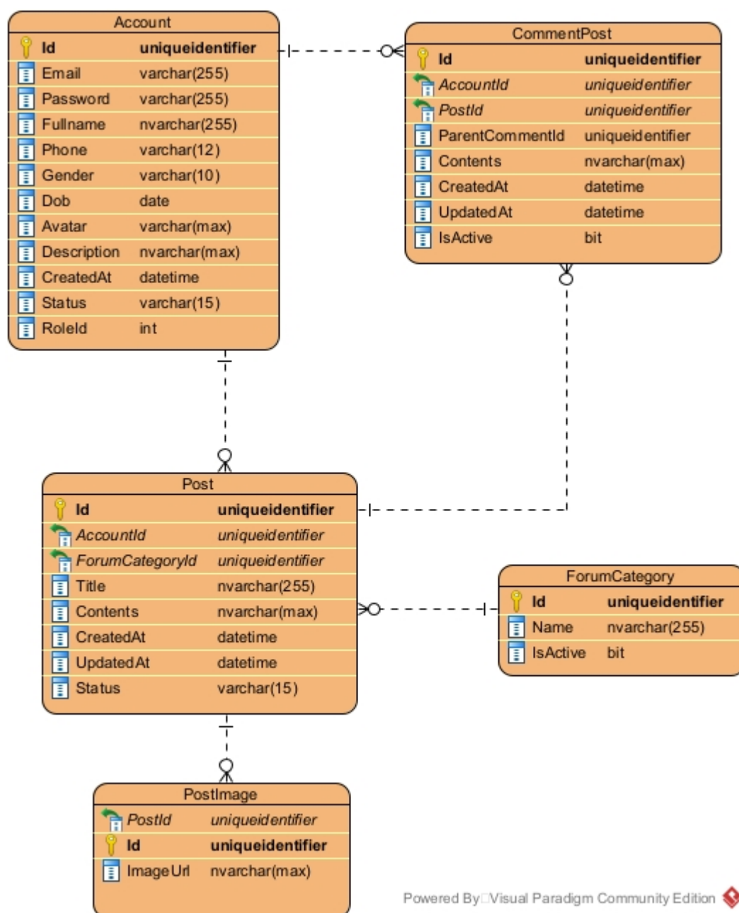
Figure 1.5.5 - Forum relationship diagram
