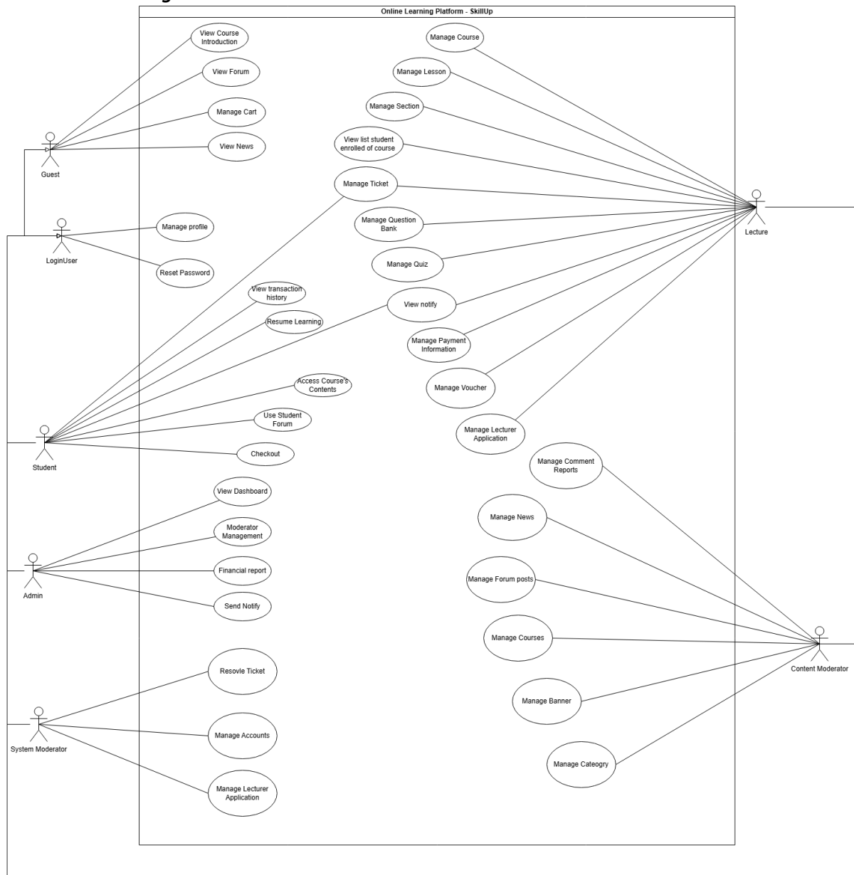
Figure 1.3.3 - Overview use case diagram
