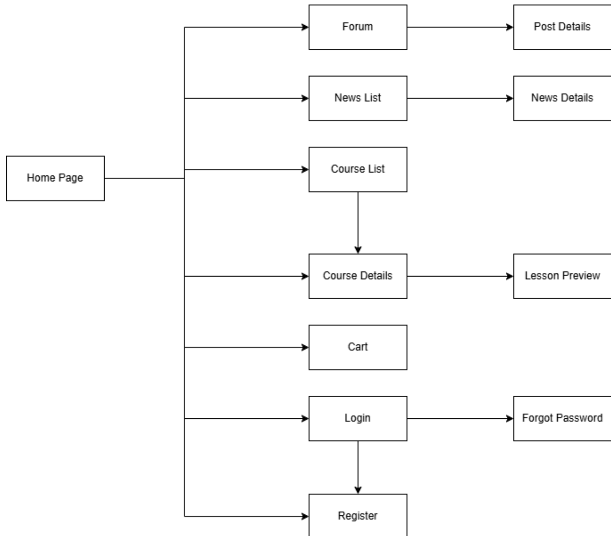
Figure 1.4.1.1 - Guest Screens Flow
