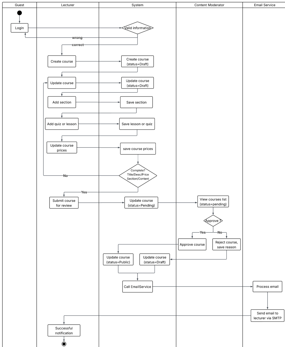
Figure 1.2.2 - Main workflow create course
