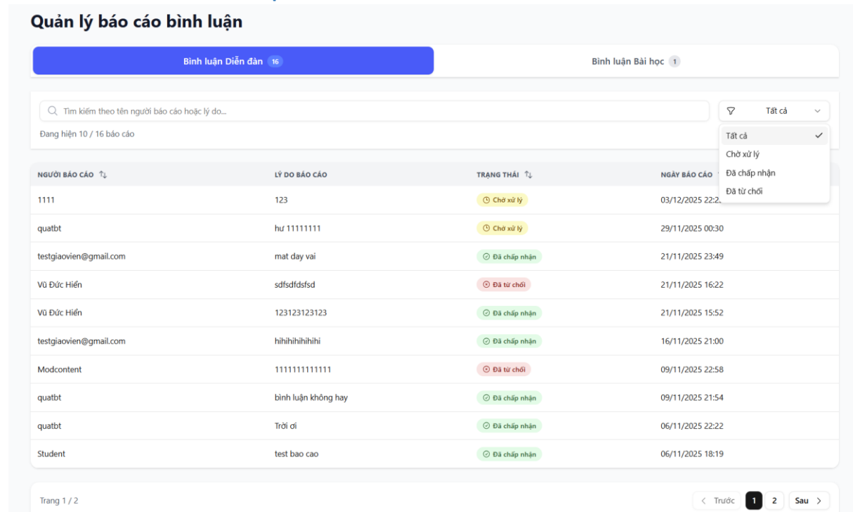
Figure 3.2.2.3 - post comment report list screen interface
