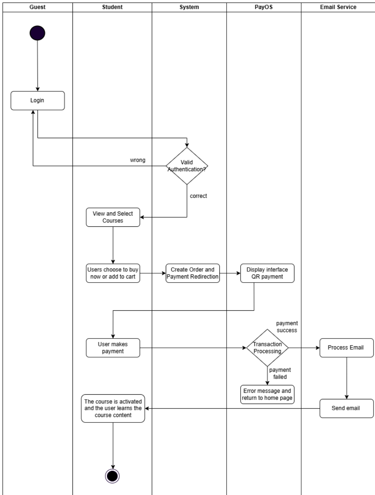
Figure 1.2.3 - Main workflow buy course and learning materials
