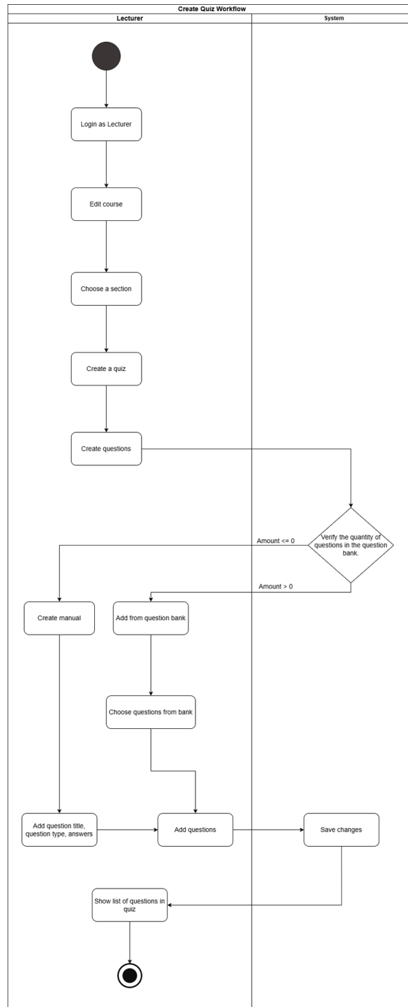
Figure 1.2.4 - Main workflow create quiz
