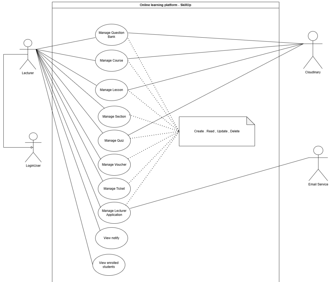
Figure 1.3.3.4 - use case lecturer diagram
