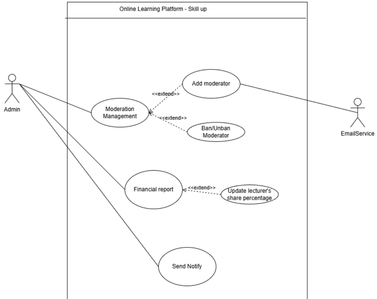
Figure 1.3.3.7 - use case admin diagram
