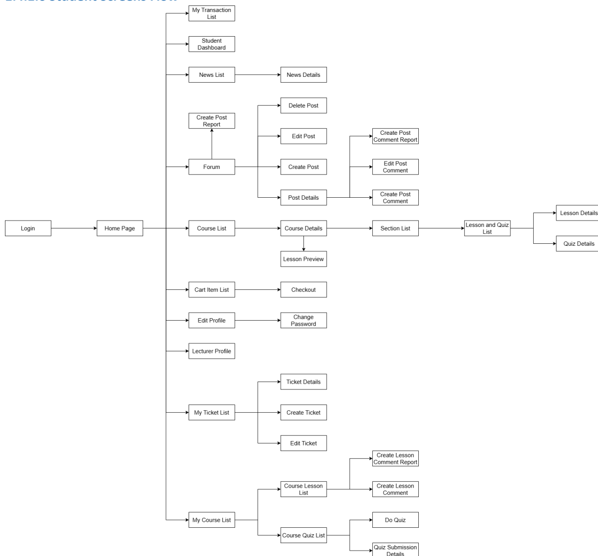
Figure 1.4.1.6 - Student Screens Flow
