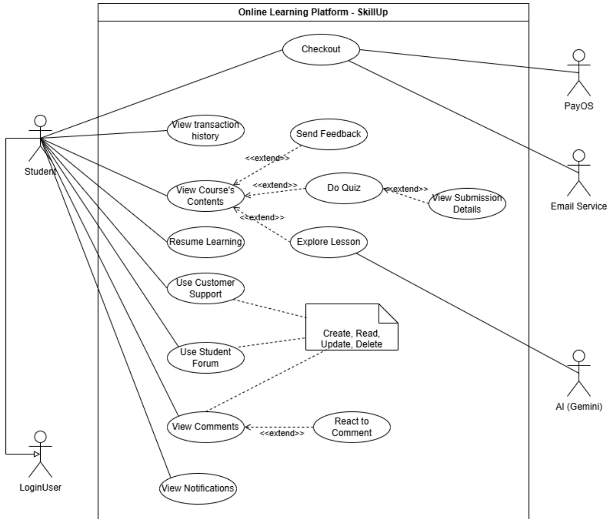
Figure 1.3.3.3 - use case student diagram
