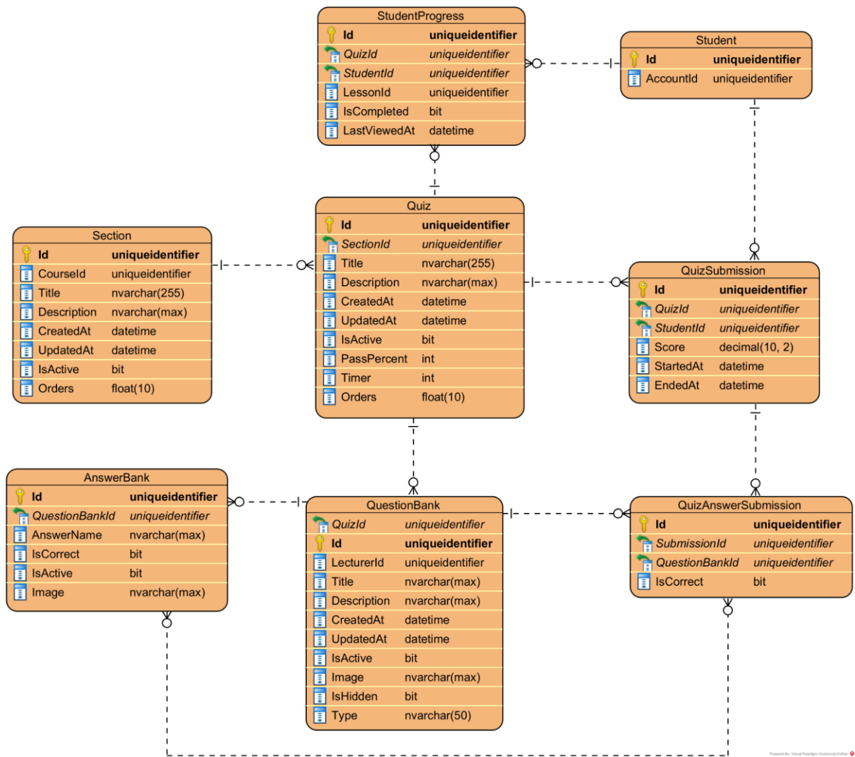
Figure 1.5.2 - Quiz entity relationship diagram
