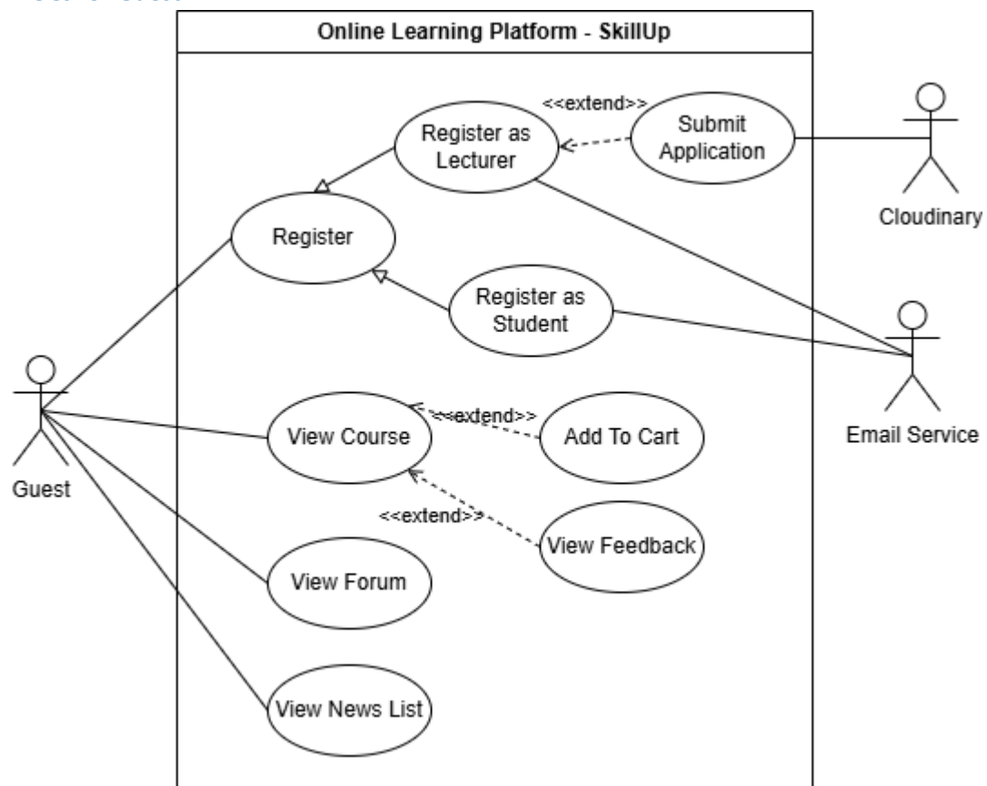
Figure 1.3.3.2 - use case guest diagram
