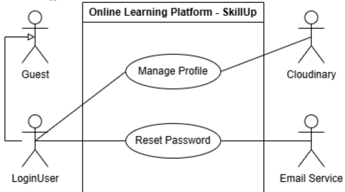
Figure 1.3.3.1 - use case logged in user diagram
